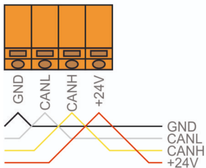
Terminals
