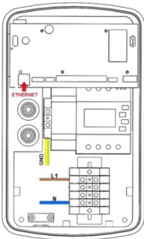
Model without RCD
