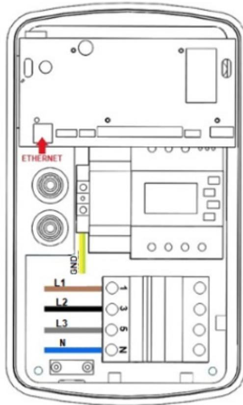
Model with RCD
