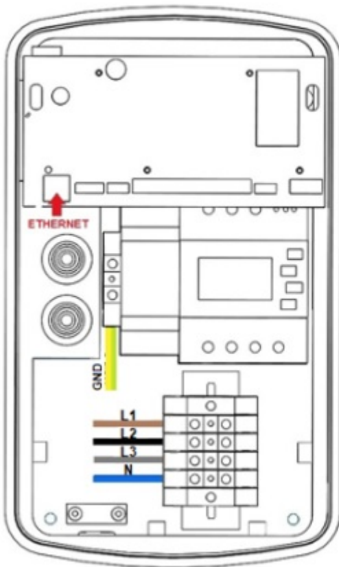
Model without RCD
